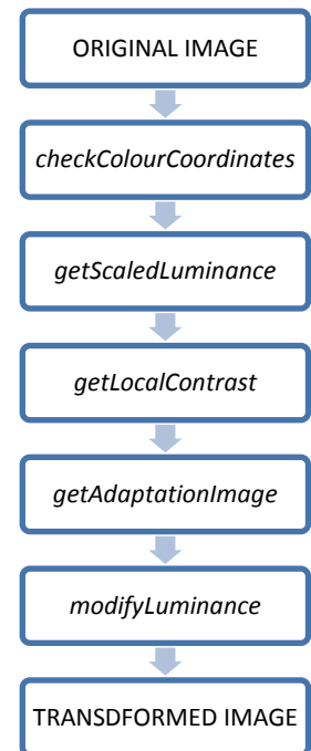
Figure 6 - Flowchart illustrating transformation of an image with Photographic Tone Reproduction
